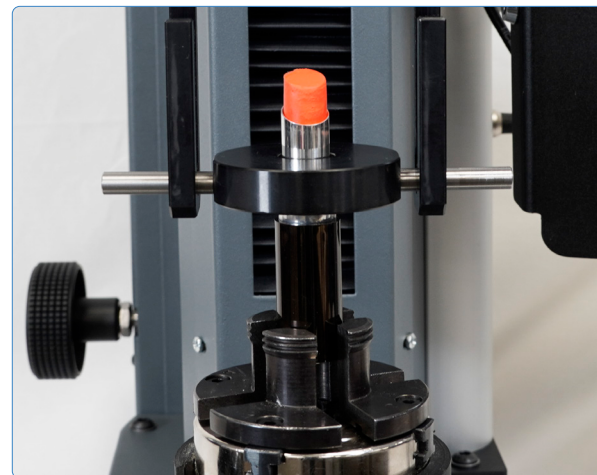
▲ Lipstick barrel rotation torque
